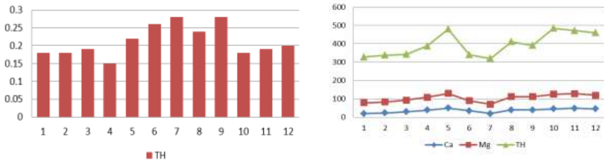
Fig 6 - The monthly changes of Dez River TH in the Year 2013 and change of Ca and MG cation values.
