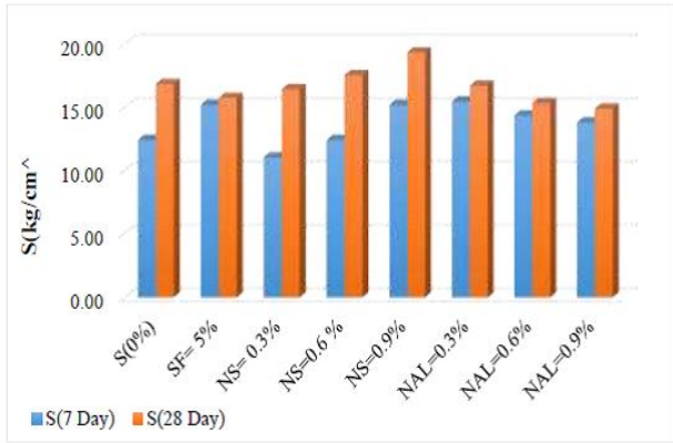
Fig.6- 7-day and 28-day compressive strength of the samples (water to cement:1/8)
