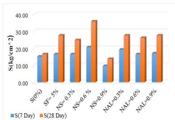
Fig.5- 7-day and 28-day compressive strength of the samples (water to cement: 1/4)
