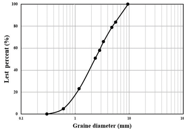
Fig.1- The grading curve
